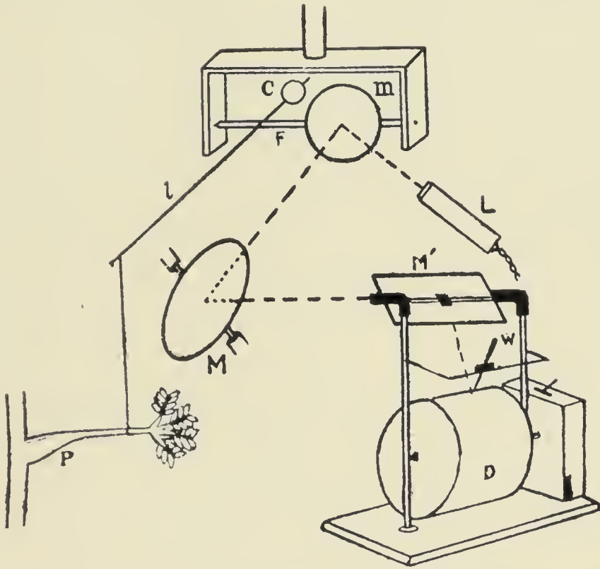
FIG. 5. The Optical Lever.
